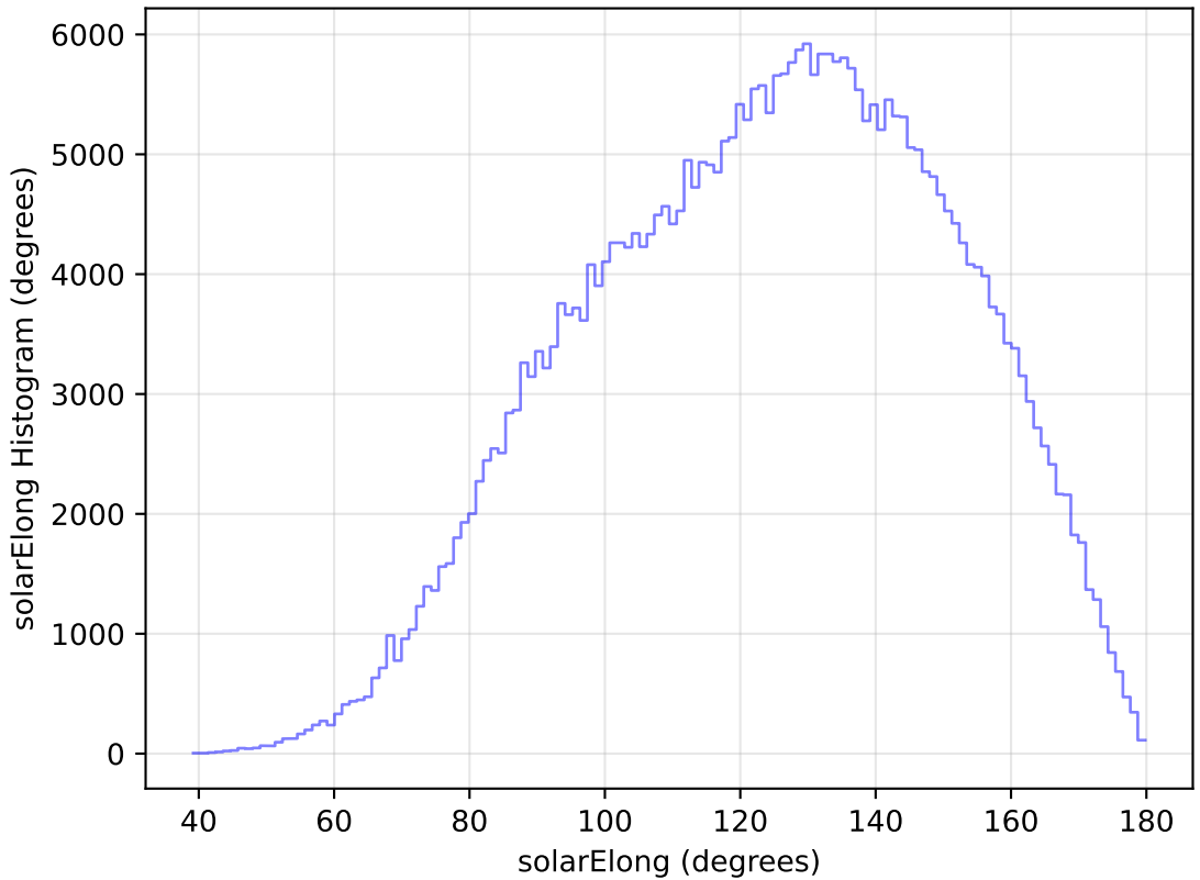
internal_u_expt60_nscale0.9v3.4_10yrs WFD y band: solarElong Histogram
