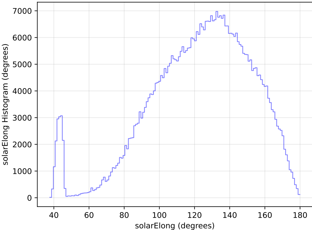
internal_u_expt60_nscale0.9v3.4_10yrs WFD r band: solarElong Histogram
