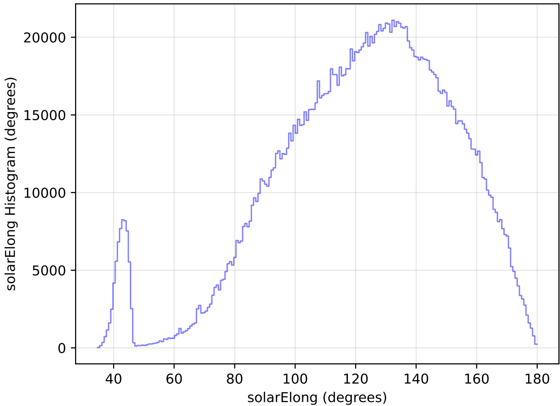
internal_u_expt60_nscale0.9v3.4_10yrs WFD all bands: solarElong Histogram
