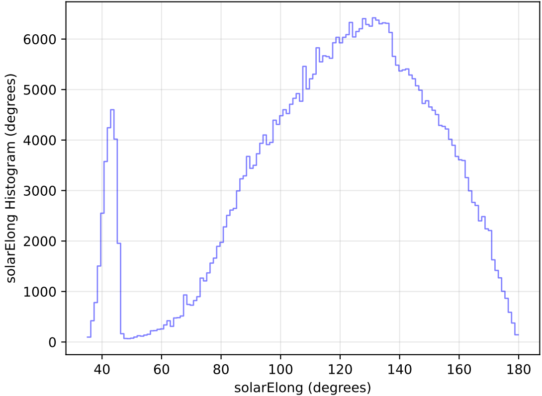
internal_u_expt60_nscale0.9v3.4_10yrs All sky z band: solarElong Histogram
