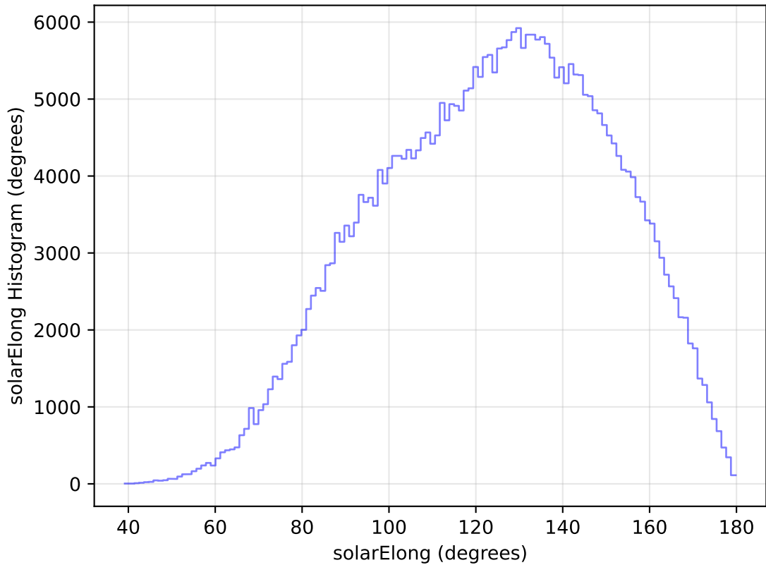
internal_u_expt60_nscale0.9v3.4_10yrs All sky y band: solarElong Histogram
