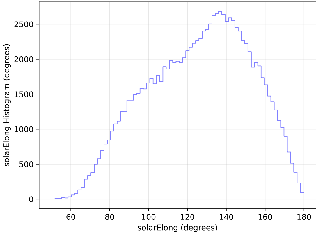
internal_u_expt60_nscale0.9v3.4_10yrs All sky u band: solarElong Histogram
