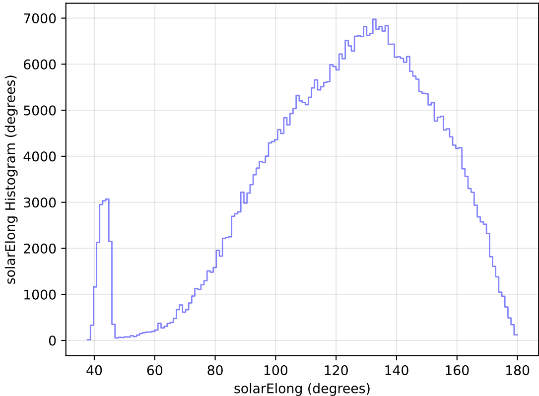
internal_u_expt60_nscale0.9v3.4_10yrs All sky r band: solarElong Histogram
