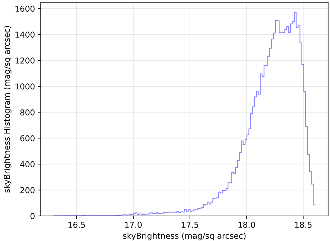
internal_u_expt60_nscale0.9v3.4_10yrs Yr 1 y band: skyBrightness Histogram
