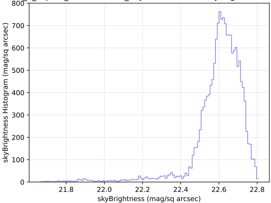
internal_u_expt60_nscale0.9v3.4_10yrs Yr 1 u band: skyBrightness Histogram
