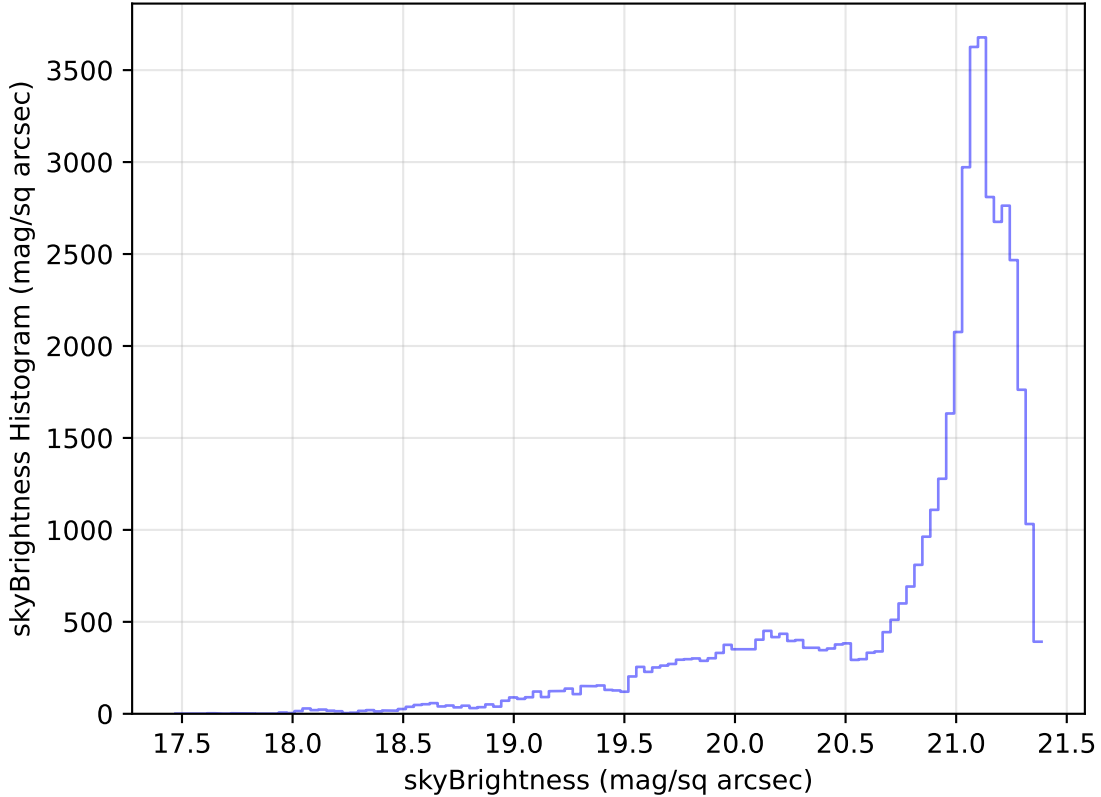
internal_u_expt60_nscale0.9v3.4_10yrs Yr 1 r band: skyBrightness Histogram
