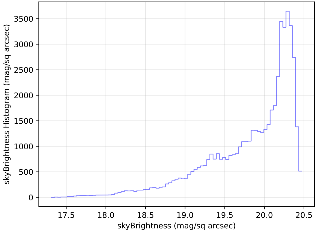
internal_u_expt60_nscale0.9v3.4_10yrs Yr 1 i band: skyBrightness Histogram
