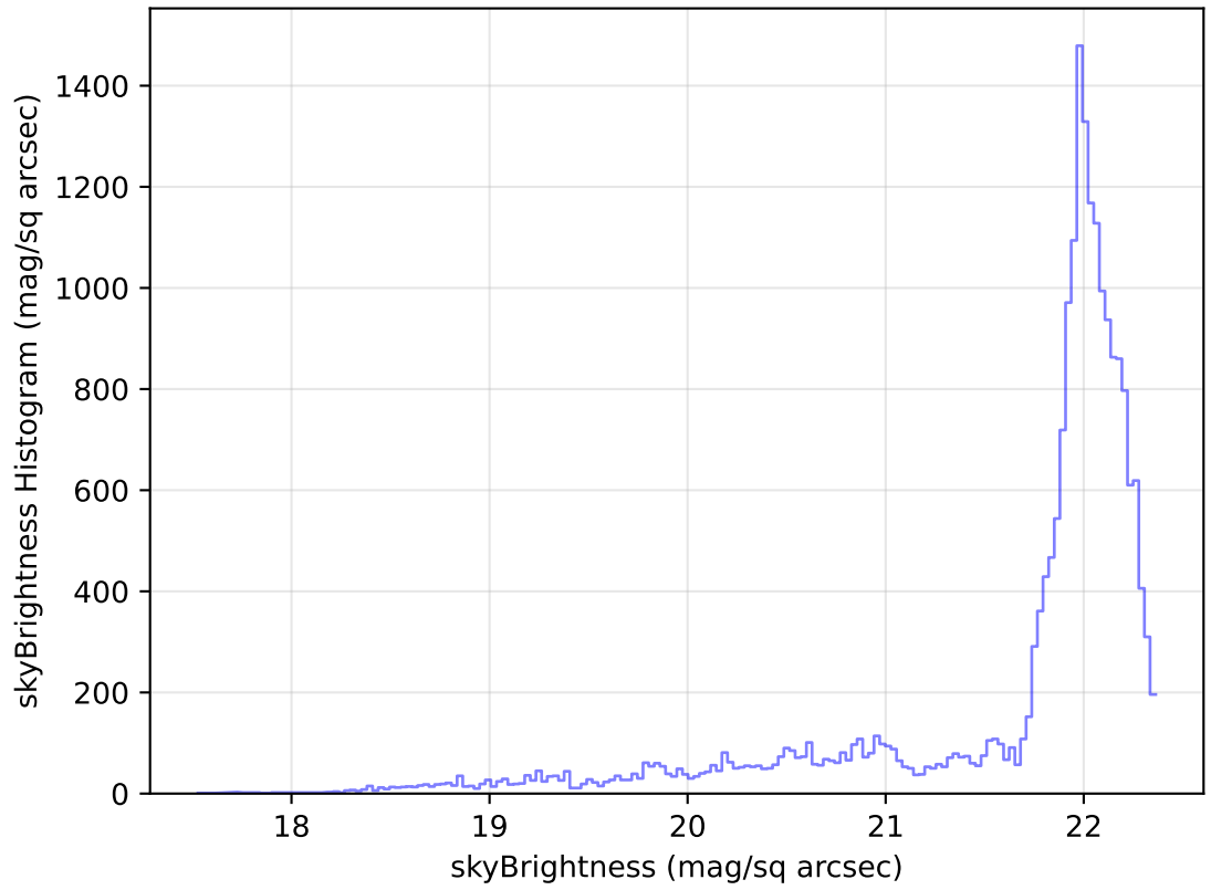
internal_u_expt60_nscale0.9v3.4_10yrs Yr 1 g band: skyBrightness Histogram
