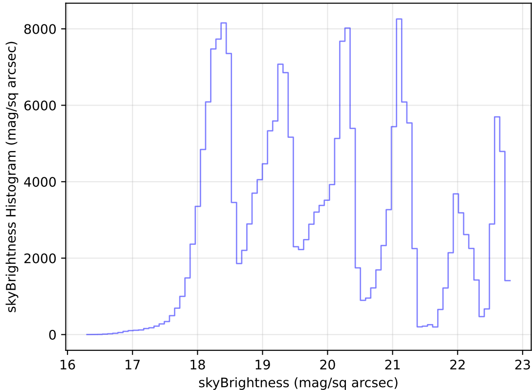
internal_u_expt60_nscale0.9v3.4_10yrs Yr 1 all bands: skyBrightness Histogram
