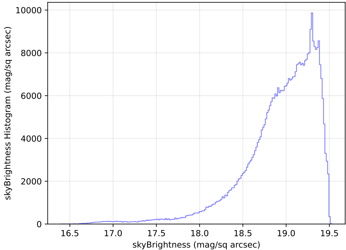
internal_u_expt60_nscale0.9v3.4_10yrs WFD z band: skyBrightness Histogram
