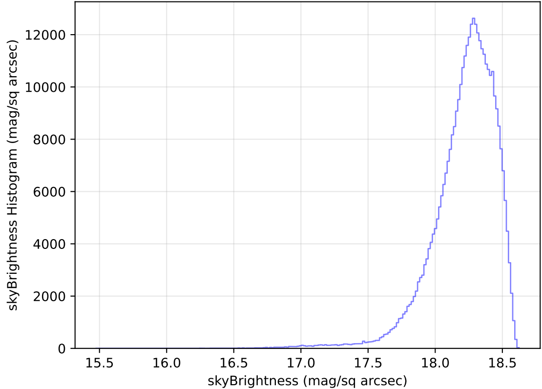
internal_u_expt60_nscale0.9v3.4_10yrs WFD y band: skyBrightness Histogram
