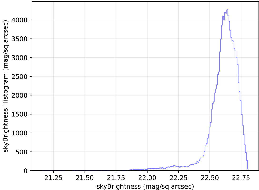
internal_u_expt60_nscale0.9v3.4_10yrs WFD u band: skyBrightness Histogram
