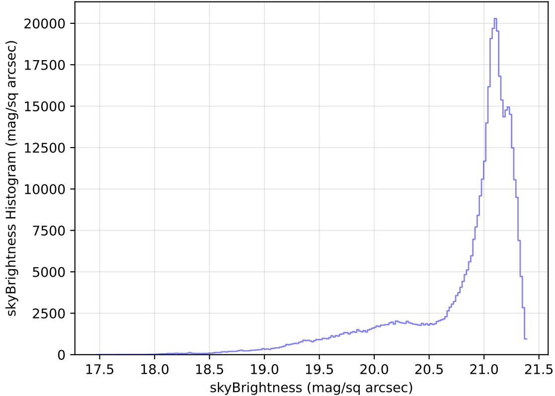
internal_u_expt60_nscale0.9v3.4_10yrs WFD r band: skyBrightness Histogram
