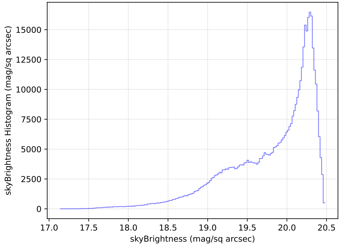
internal_u_expt60_nscale0.9v3.4_10yrs WFD i band: skyBrightness Histogram
