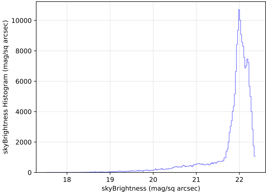
internal_u_expt60_nscale0.9v3.4_10yrs WFD g band: skyBrightness Histogram
