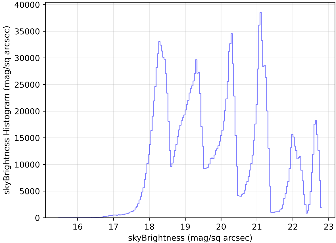
internal_u_expt60_nscale0.9v3.4_10yrs WFD all bands: skyBrightness Histogram
