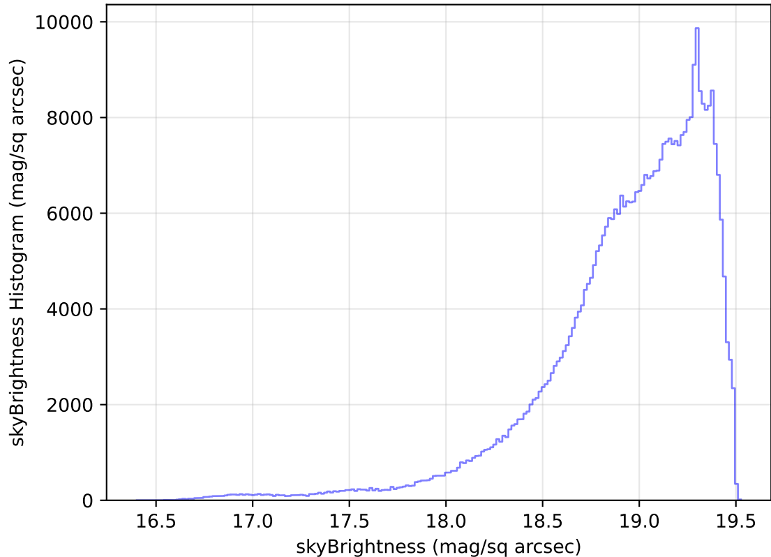
internal_u_expt60_nscale0.9v3.4_10yrs All sky z band: skyBrightness Histogram
