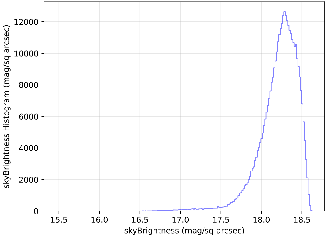
internal_u_expt60_nscale0.9v3.4_10yrs All sky y band: skyBrightness Histogram
