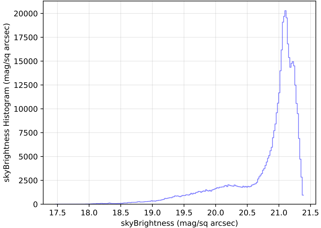
internal_u_expt60_nscale0.9v3.4_10yrs All sky r band: skyBrightness Histogram
