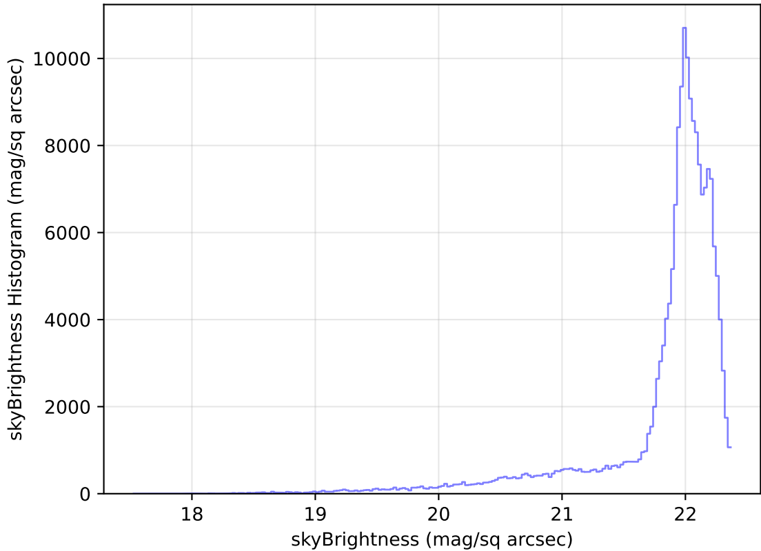
internal_u_expt60_nscale0.9v3.4_10yrs All sky g band: skyBrightness Histogram
