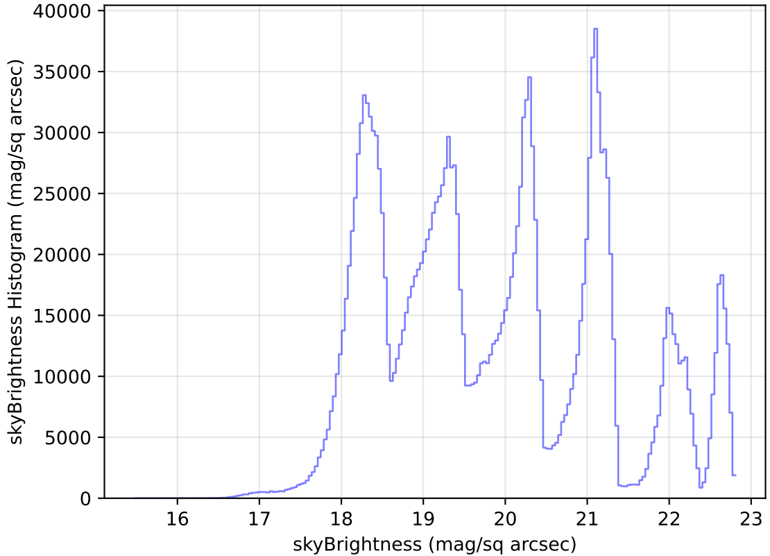
internal_u_expt60_nscale0.9v3.4_10yrs All sky all bands: skyBrightness Histogram
