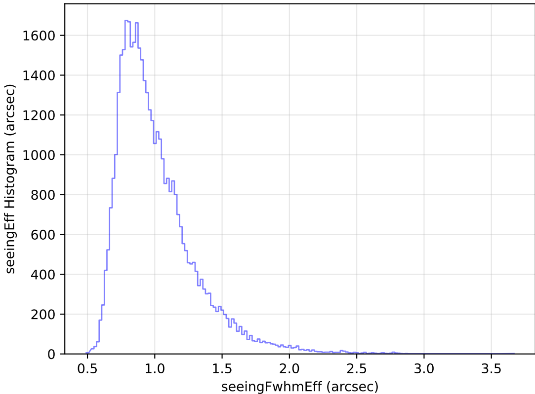
internal_u_expt60_nscale0.9v3.4_10yrs Yr 1 z band: seeingEff Histogram
