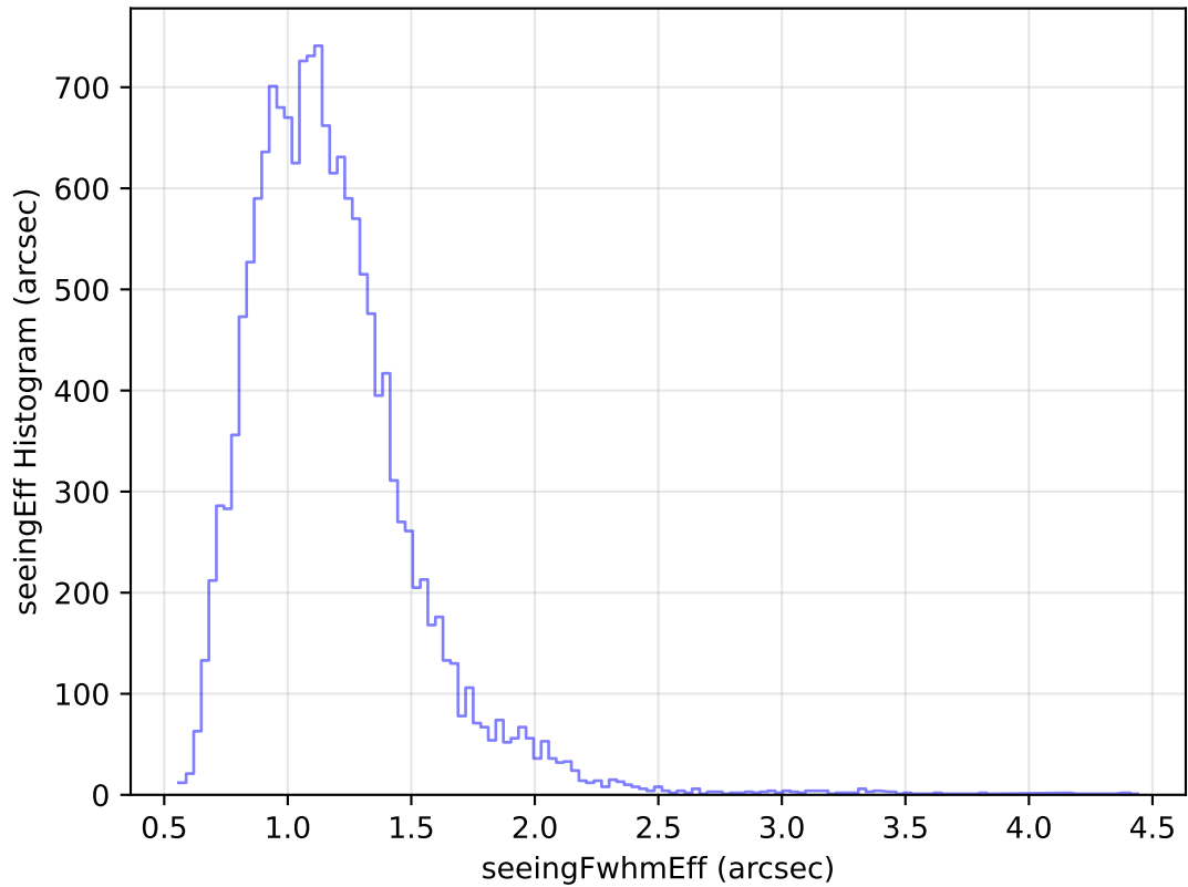
internal_u_expt60_nscale0.9v3.4_10yrs Yr 1 u band: seeingEff Histogram
