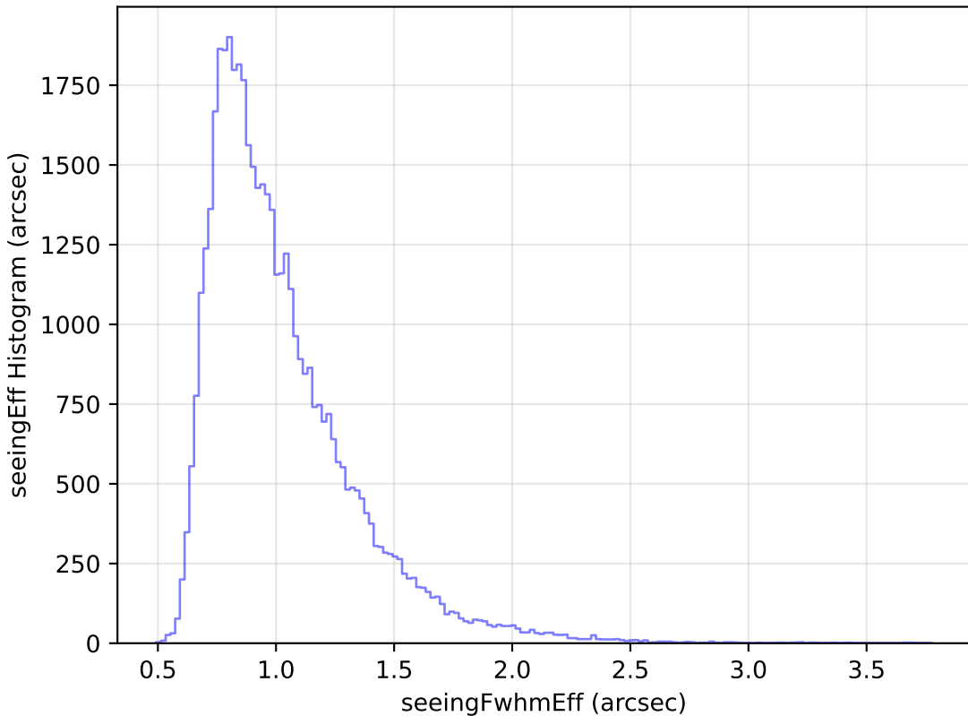
internal_u_expt60_nscale0.9v3.4_10yrs Yr 1 r band: seeingEff Histogram
