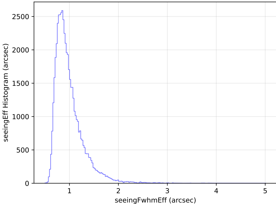
internal_u_expt60_nscale0.9v3.4_10yrs Yr 1 i band: seeingEff Histogram
