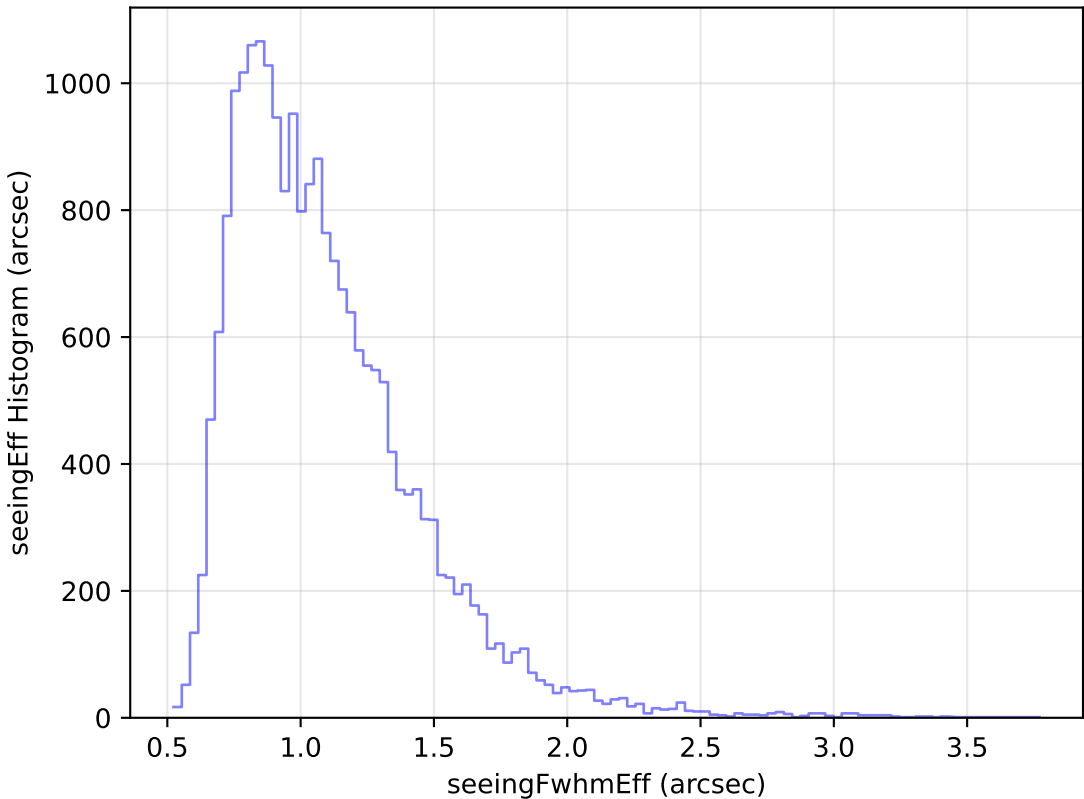
internal_u_expt60_nscale0.9v3.4_10yrs Yr 1 g band: seeingEff Histogram
