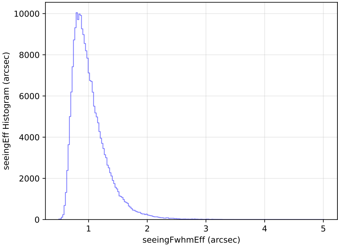
internal_u_expt60_nscale0.9v3.4_10yrs Yr 1 all bands: seeingEff Histogram
