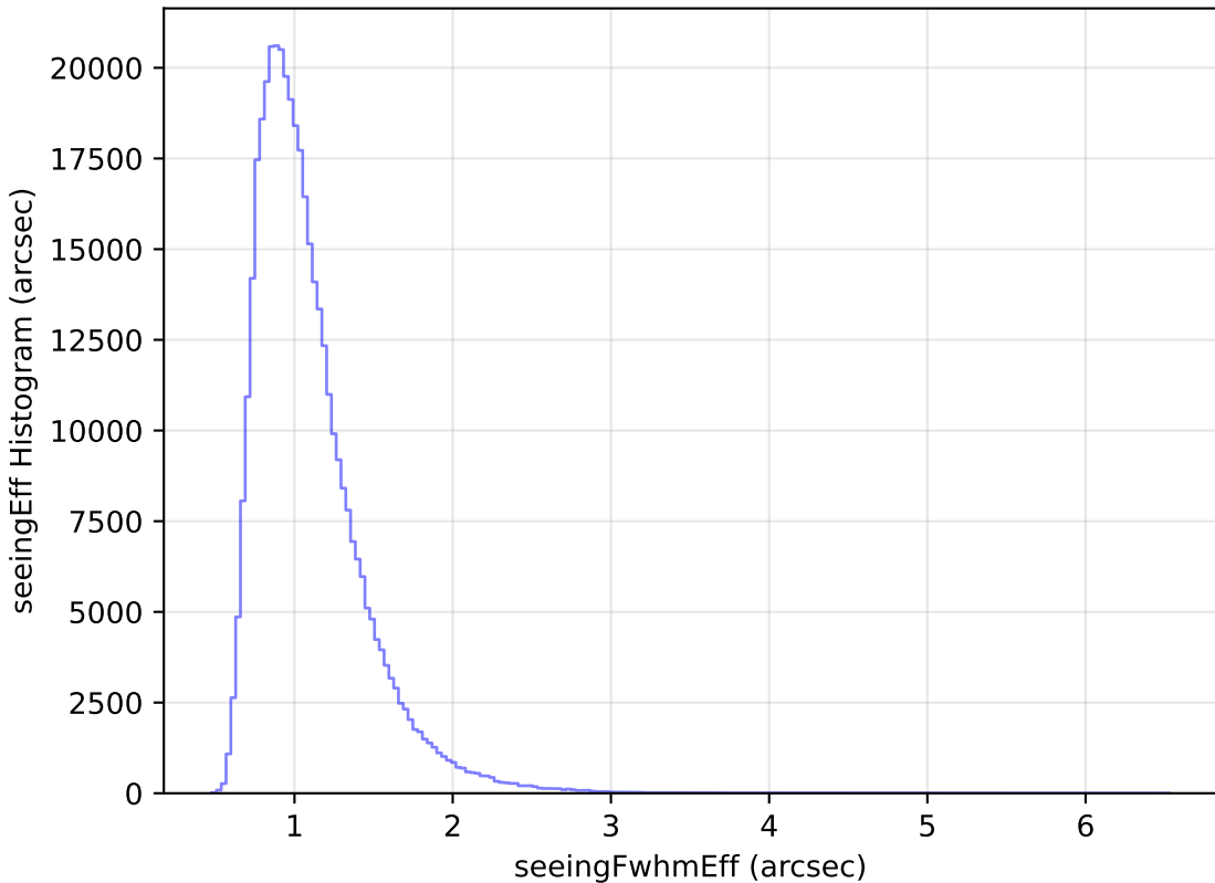
internal_u_expt60_nscale0.9v3.4_10yrs WFD z band: seeingEff Histogram
