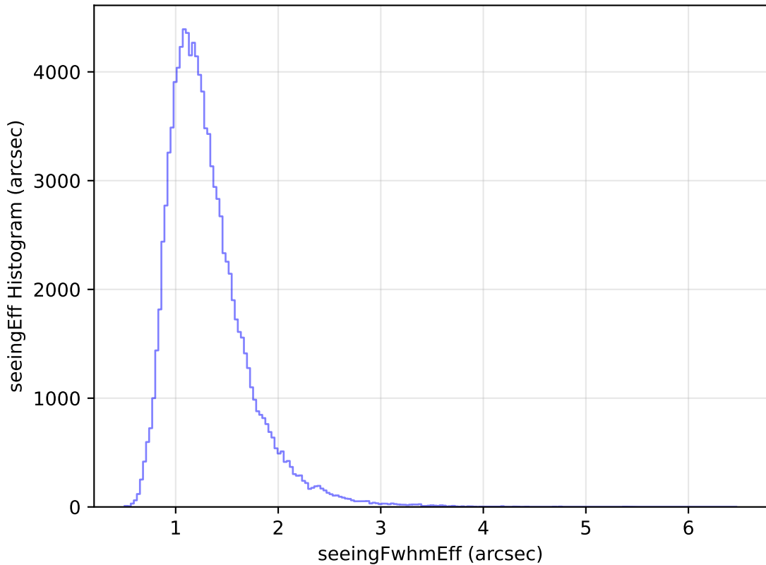
internal_u_expt60_nscale0.9v3.4_10yrs WFD u band: seeingEff Histogram
