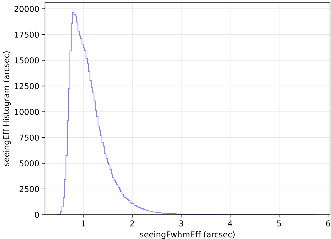
internal_u_expt60_nscale0.9v3.4_10yrs WFD r band: seeingEff Histogram
