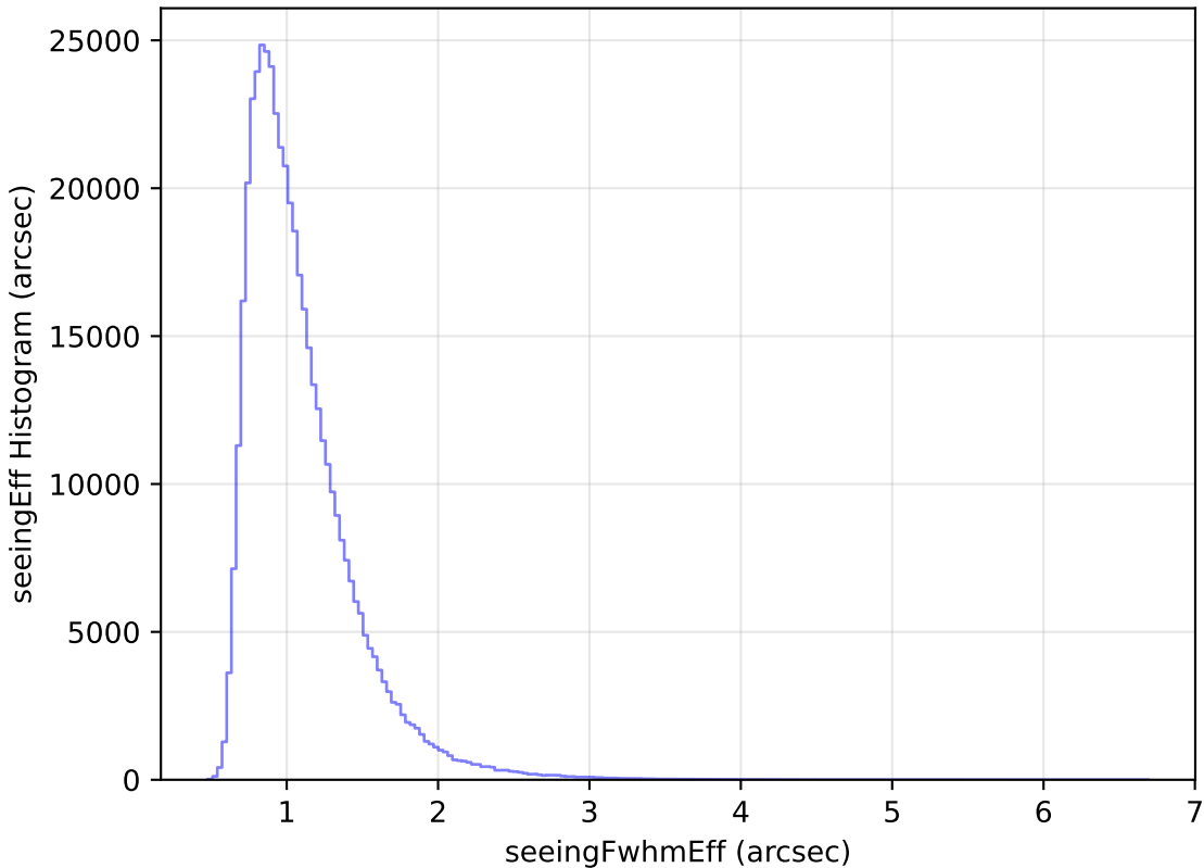
internal_u_expt60_nscale0.9v3.4_10yrs WFD i band: seeingEff Histogram
