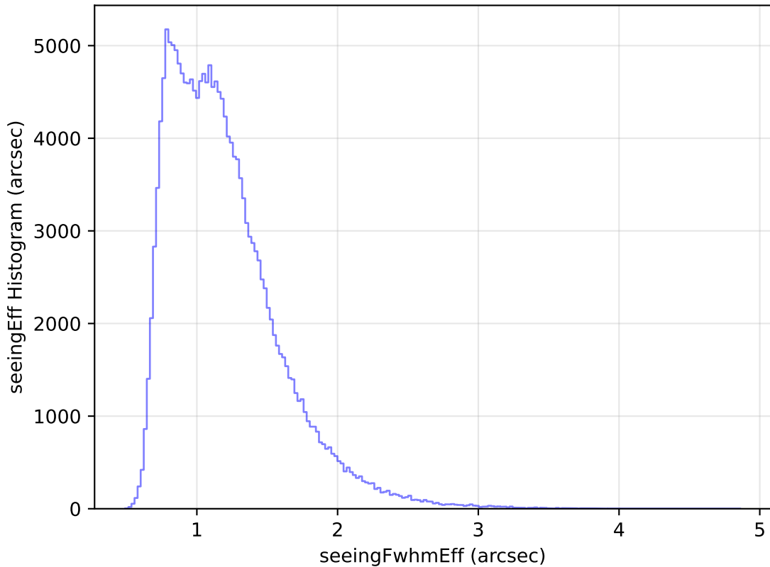
internal_u_expt60_nscale0.9v3.4_10yrs WFD g band: seeingEff Histogram
