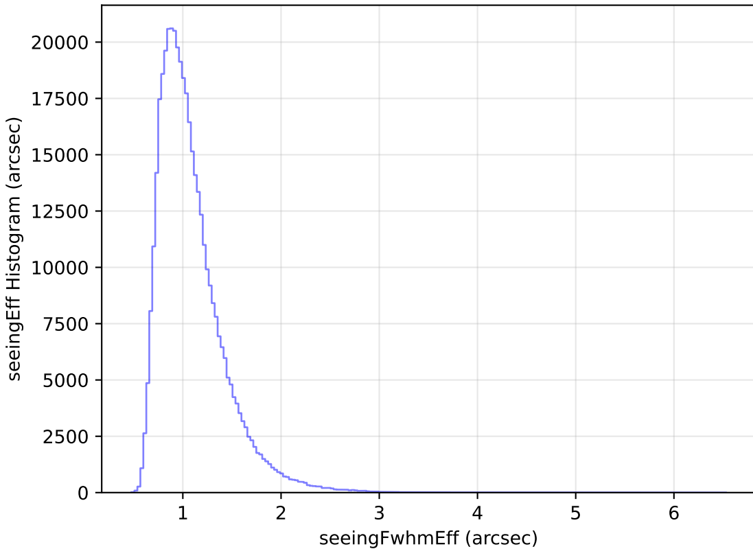
internal_u_expt60_nscale0.9v3.4_10yrs All sky z band: seeingEff Histogram
