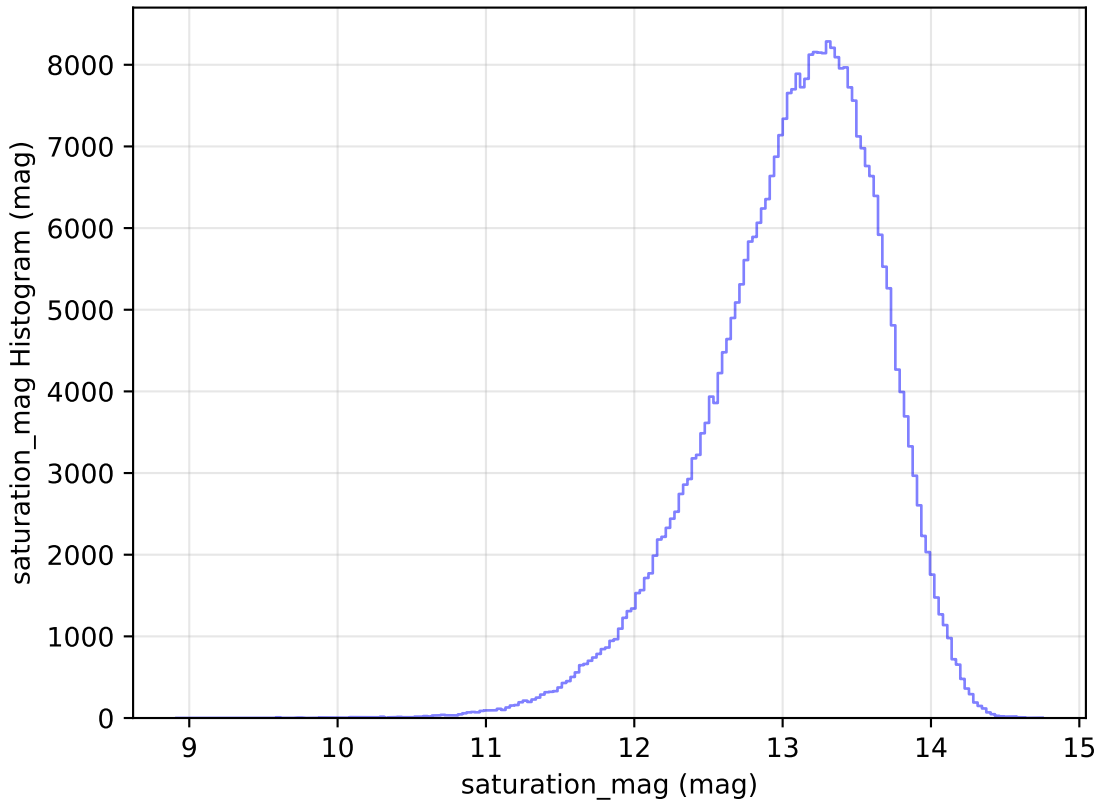
internal_u_expt60_nscale0.9v3.4_10yrs WFD y band: saturation_mag Histogram
