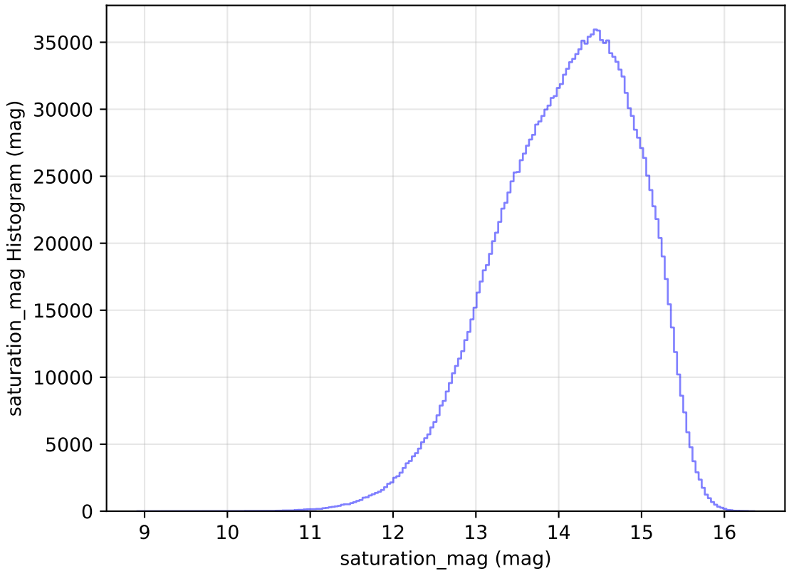
internal_u_expt60_nscale0.9v3.4_10yrs WFD all bands: saturation_mag Histogram
