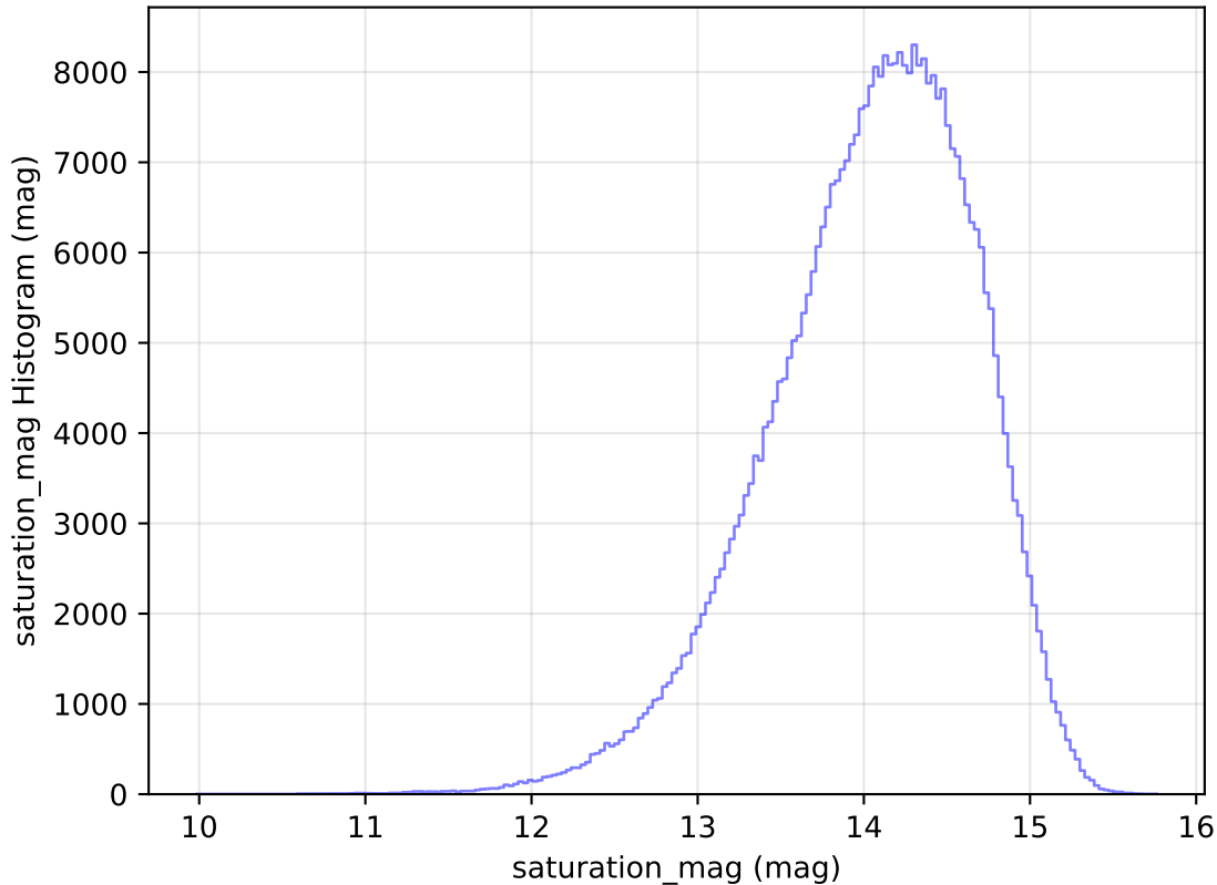
internal_u_expt60_nscale0.9v3.4_10yrs All sky z band: saturation_mag Histogram
