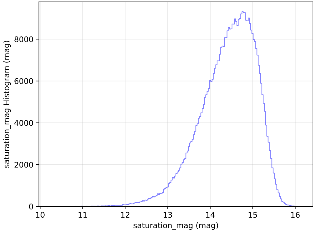
internal_u_expt60_nscale0.9v3.4_10yrs All sky i band: saturation_mag Histogram
