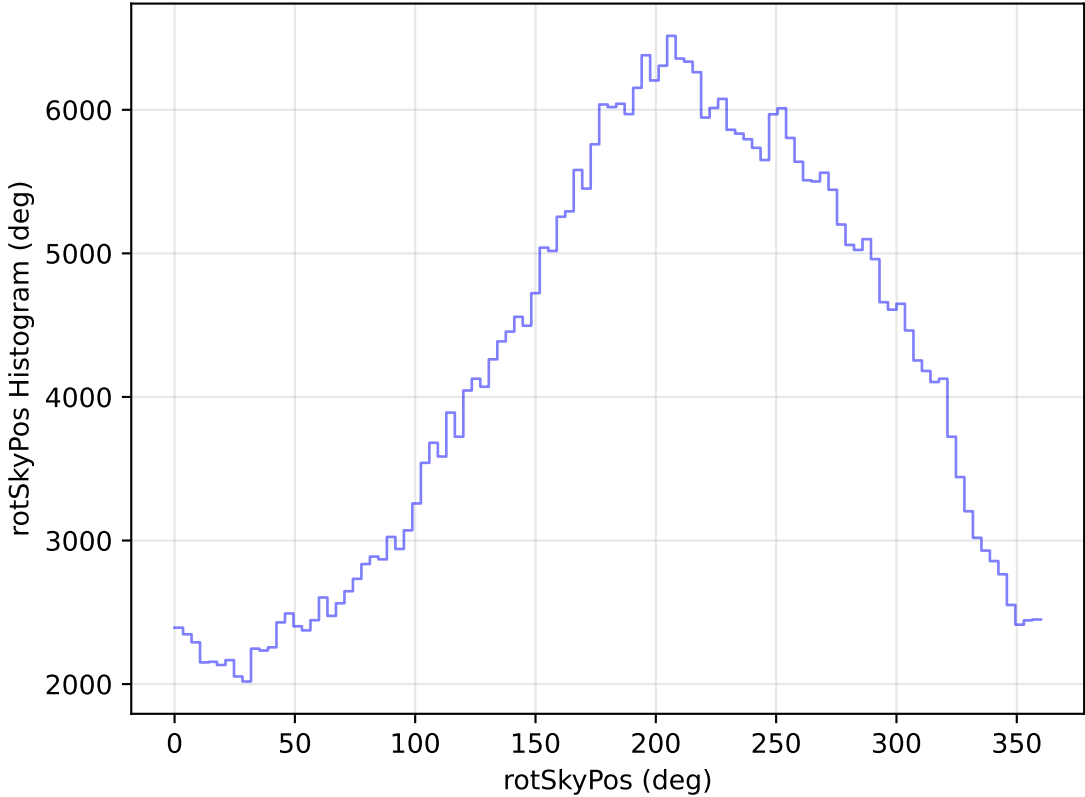
internal_u_expt60_nscale0.9v3.4_10yrs WFD z band: rotSkyPos Histogram
