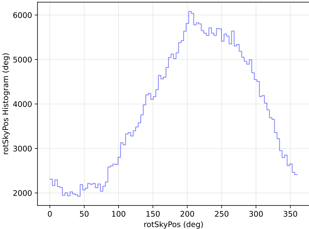
internal_u_expt60_nscale0.9v3.4_10yrs WFD y band: rotSkyPos Histogram
