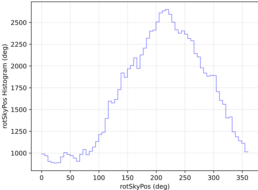
internal_u_expt60_nscale0.9v3.4_10yrs WFD u band: rotSkyPos Histogram
