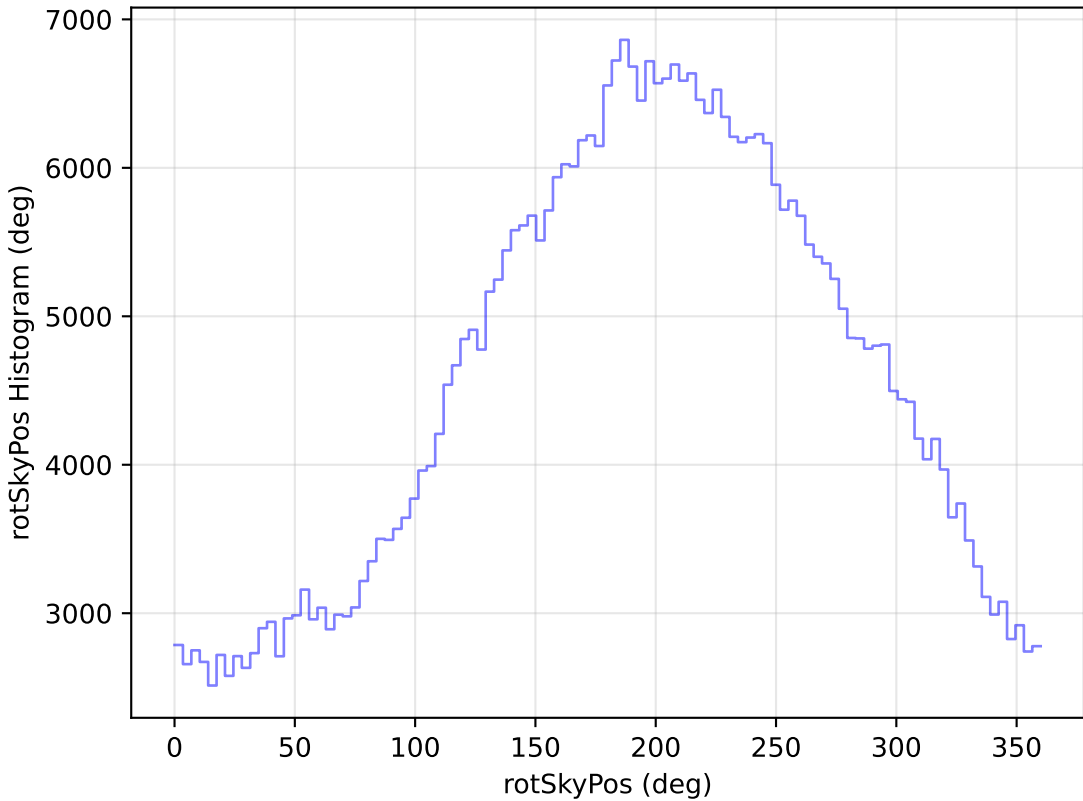
internal_u_expt60_nscale0.9v3.4_10yrs WFD r band: rotSkyPos Histogram
