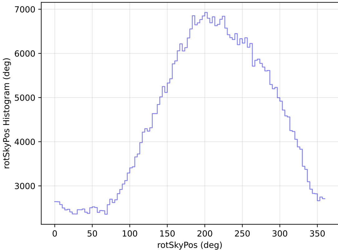
internal_u_expt60_nscale0.9v3.4_10yrs WFD i band: rotSkyPos Histogram
