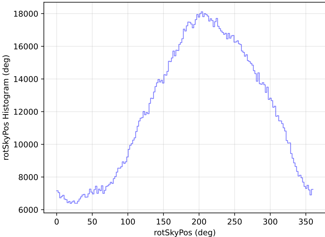
internal_u_expt60_nscale0.9v3.4_10yrs WFD all bands: rotSkyPos Histogram
