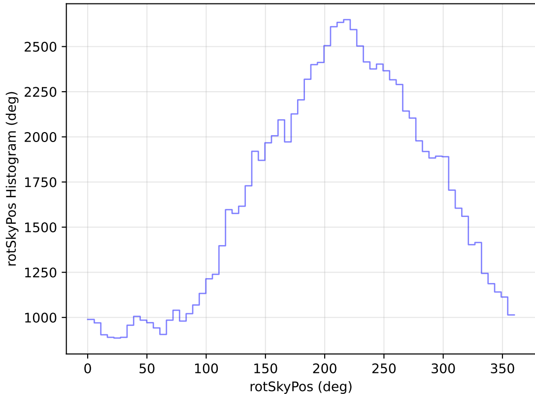
internal_u_expt60_nscale0.9v3.4_10yrs All sky u band: rotSkyPos Histogram
