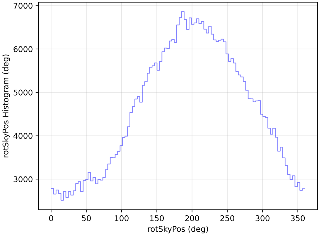
internal_u_expt60_nscale0.9v3.4_10yrs All sky r band: rotSkyPos Histogram
