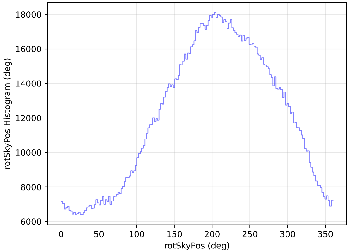
internal_u_expt60_nscale0.9v3.4_10yrs All sky all bands: rotSkyPos Histogram
